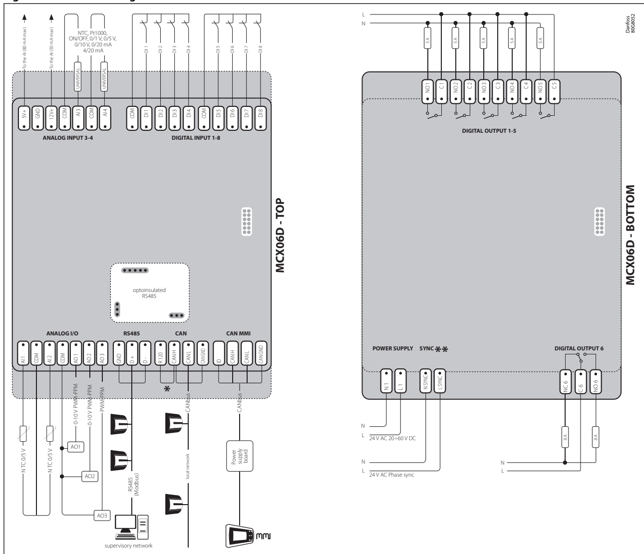
Figure 1: Connection diagram
